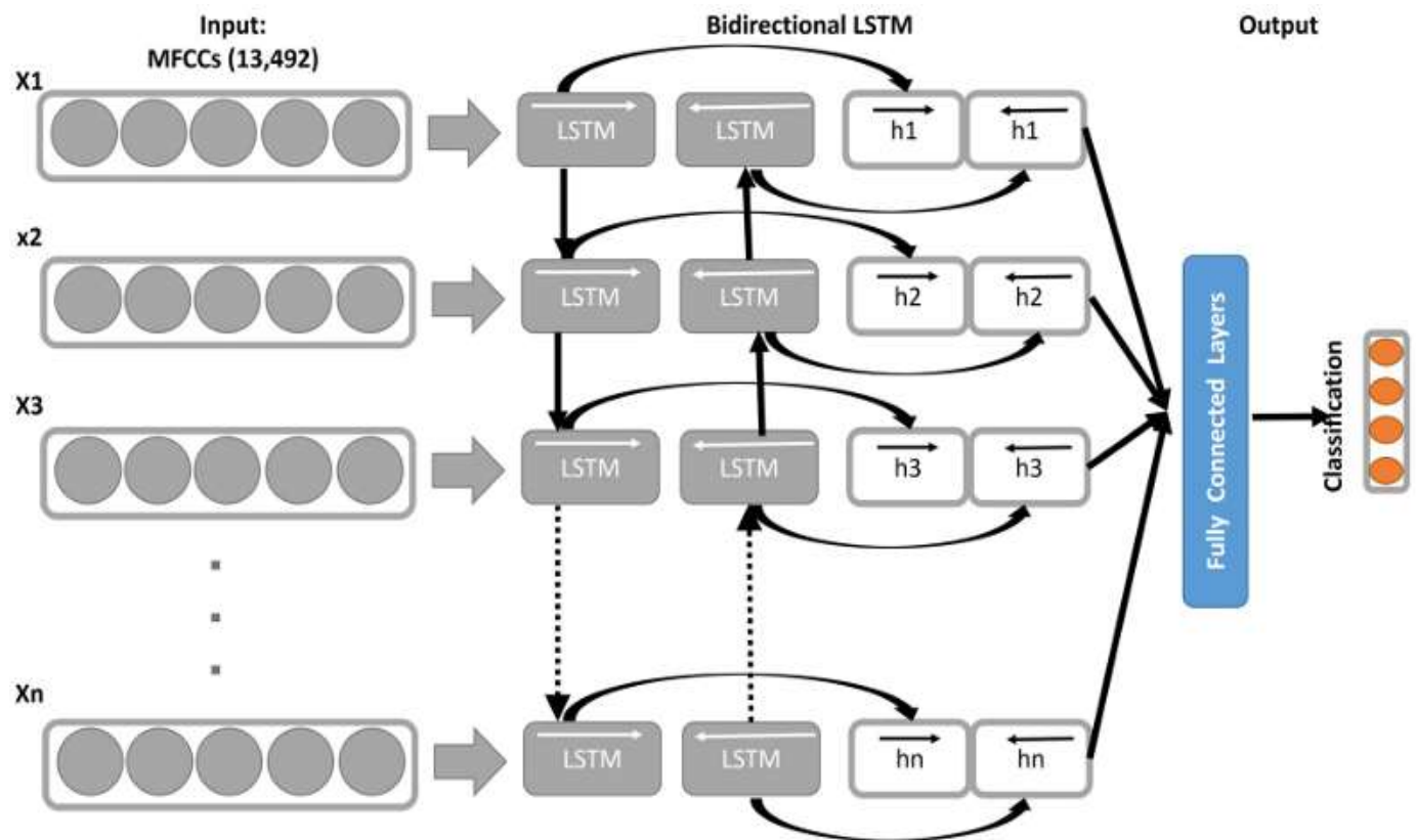
Figure 8. Bi-LSTM architecture with 50 Bi-LSTM layers and fully connected layers [21]
