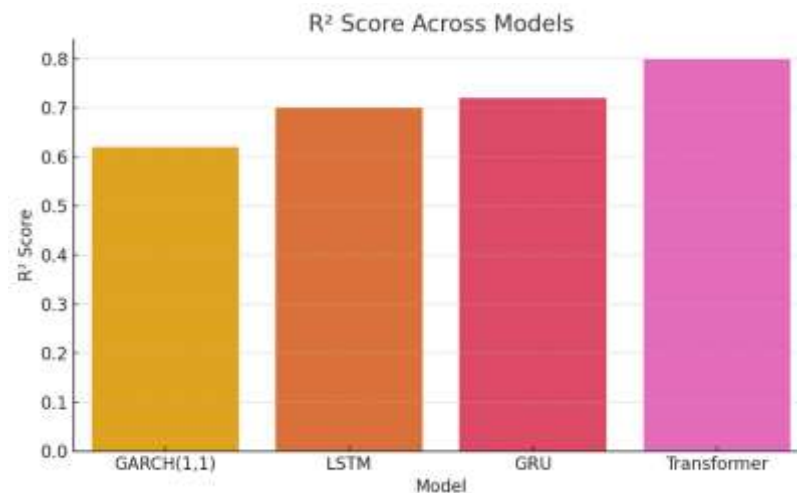
Figure 3: Comparison of R^2 Score Across Models
