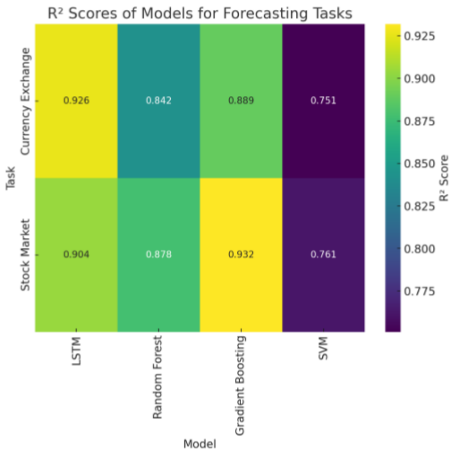
Figure 5: A heatmap visualizing the R2R^2R2 scores of the models for both forecasting tasks, highlighting model performance differences.
